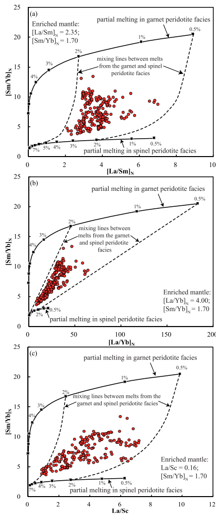
Figure 8. (a) [\text{Sm}/\text{Yb}]_N versus [\text{La}/\text{Sm}]_N , (b) [\text{Sm}/\text{Yb}]_N versus [\text{La}/\text{Yb}]_N , and (c) [\text{Sm}/\text{Yb}]_N versus \text{La}/\text{Sc} for the Cenozoic basalts in eastern China. The solid curves show non-modal fractional melting models in the garnet and spinel peridotite facies, respectively. The dashed curves show mixing trends between a 0.5% melt from the garnet peridotite facies and a 2% melt from the spinel peridotite facies and between a 2% melt from the garnet peridotite facies and a 7% melt from the spinel peridotite facies, respectively. The source and melt mineral modes in garnet and spinel peridotite facies are from the compilation in Johnson (1998). Partition coefficients are from the compilation in Niu et al. (1996). The source mantle of the Cenozoic basalts in eastern China was suggested to have fertile major element compositions similar to the primitive mantle (PM) (e.g., Wu et al., 2006; Xu et al., 2000) but is more enriched in progressively more incompatible elements, which is consistent with a low-degree melt metasomatism in the low velocity zone (LVZ) prior to the major melting event (e.g., Guo et al., 2016; Niu, 2005; Sun et al., 2017). Therefore, the enriched source mantle of the Cenozoic basalts in eastern China is estimated to be a mixture of PM with 5% of a low-degree (0.5%) melt from the PM. This source mantle composition can well explain the high [\text{La}/\text{Sm}]_N (an indicator of the source enrichment) of these basalts. The PM composition is from McDonough and Sun (1995). This partial melting modeling shows that these basalts represent mixing between small melt fractions from the garnet peridotite facies with high [\text{Sm}/\text{Yb}]_N , [\text{La}/\text{Yb}]_N , and \text{La}/\text{Sc} ratios and relatively larger melt fractions from spinel peridotite facies with lower [\text{Sm}/\text{Yb}]_N , [\text{La}/\text{Yb}]_N , and \text{La}/\text{Sc} ratios.
